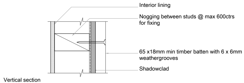
SC011 Shadowclad Vertical Joint with Optional Cover Batten (Direct)
